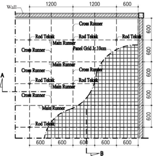
GRID CEILING INSTALLATION
